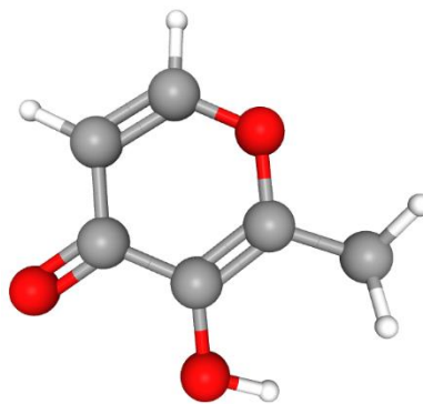
Maltol
