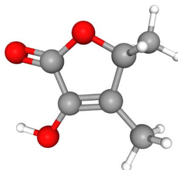
4-hydroxy-(2,3)-diméthyl-5-furanone
