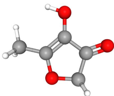
4-hydroxy-5-méthyl-3-furanone
