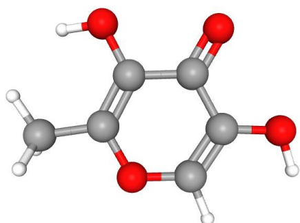
5-hydroxymaltol
