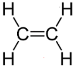
Ethylène
