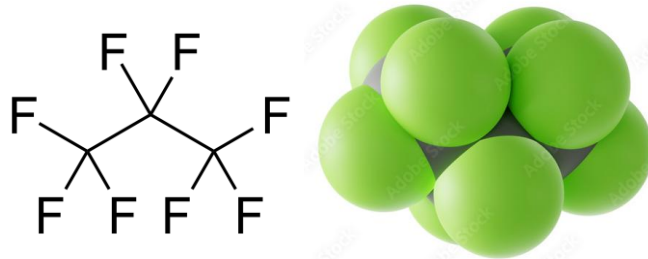
octafluoropropane \text{C}_3\text{F}_8
